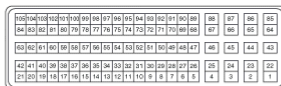
CNG-AA ECM
